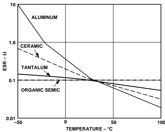
Figure 13. ESR vs. Temperature
